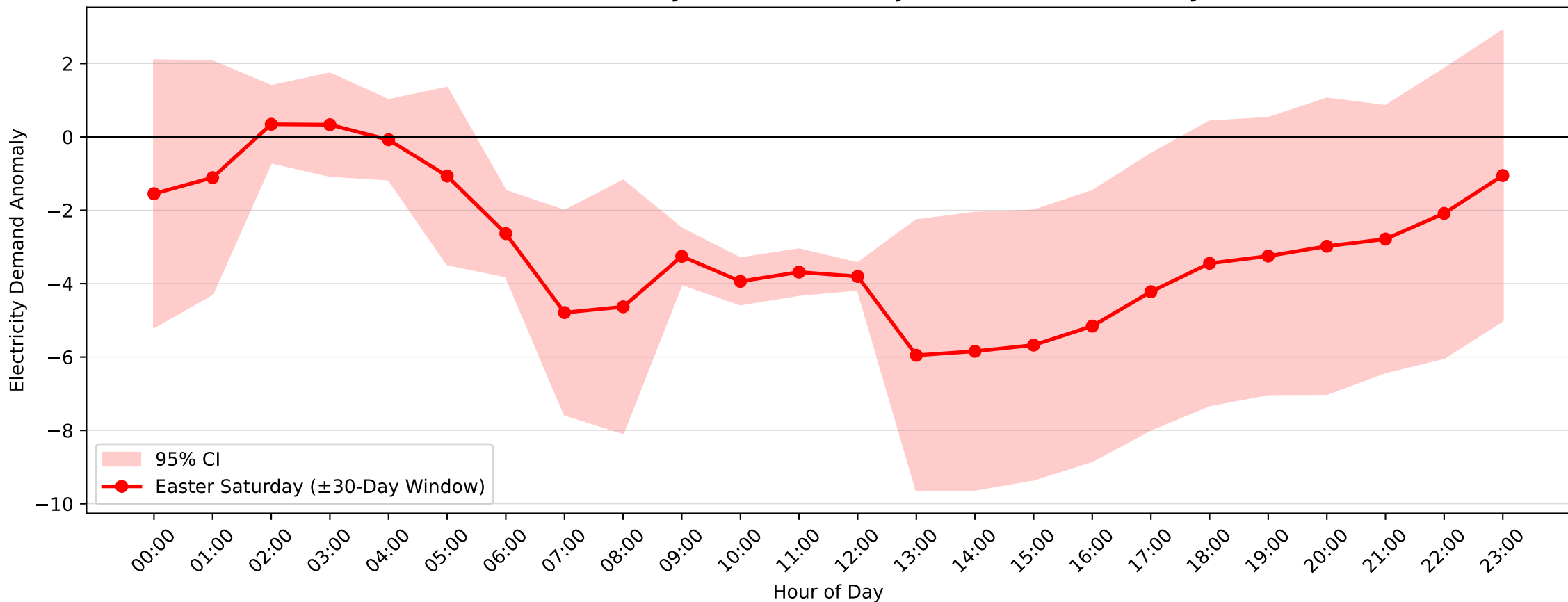
Potts Hill Demand Anomaly: Easter Saturday (2004-2017, \pm 30 -Day Window)
